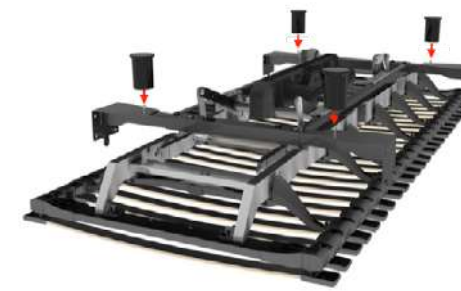
Preassembled cross bars, legs to be screwed
